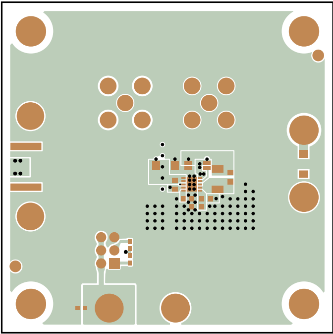
Figure 8. Example DFN Layout
